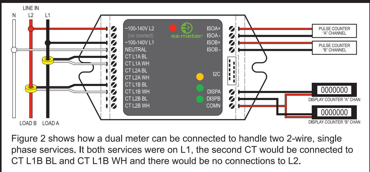
Fig. 2: Dual Output, 2-Wire, Single Element, Single Phase Meter (Type A4)
