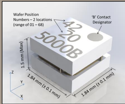
AT-5000-B Device Dimensions
