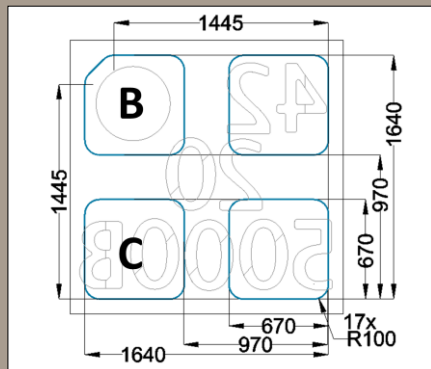
AT-5000-B Pad Dimensions (micrometers) as viewed from pad side of device
